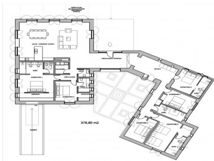
Plans groundfloor
