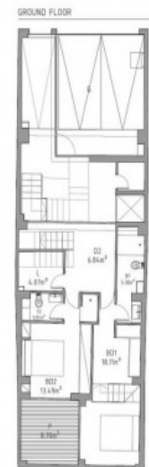
Construction plan of the lower floor
